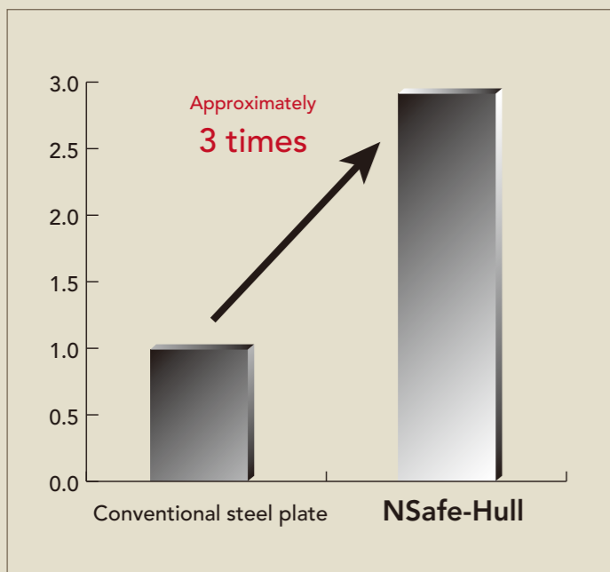
Absorbed Energy by Struck Ship, Normalised
